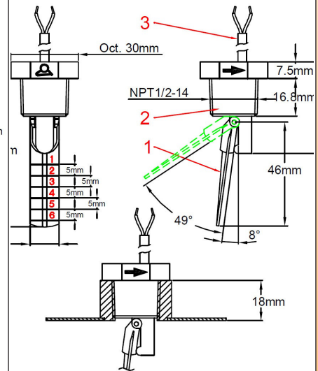
1: Palette 2: Corps 3: Cable R1F (½"NPT)
